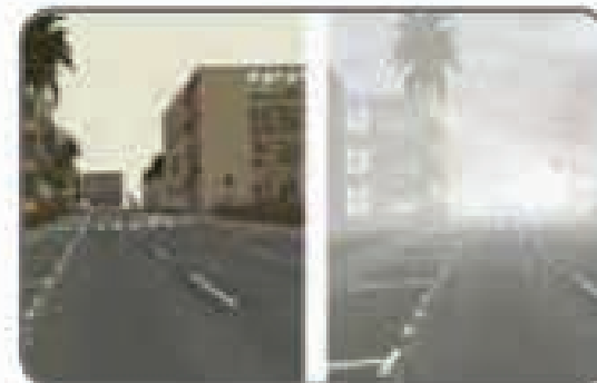
IMAGE ENHANCEMENT
