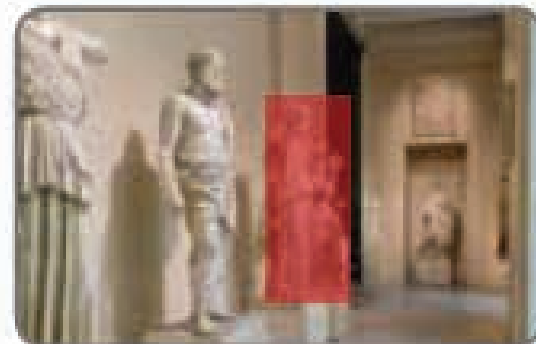
OBJECT REMOVAL
