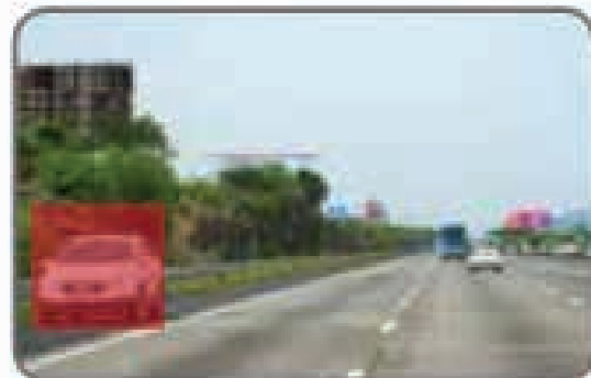
STOPPED VEHICLE
