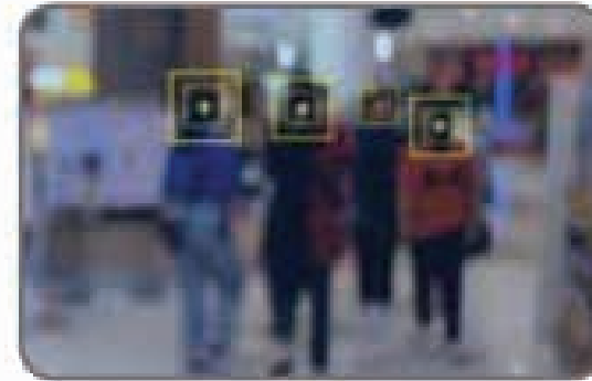
PEOPLE COUNTING
